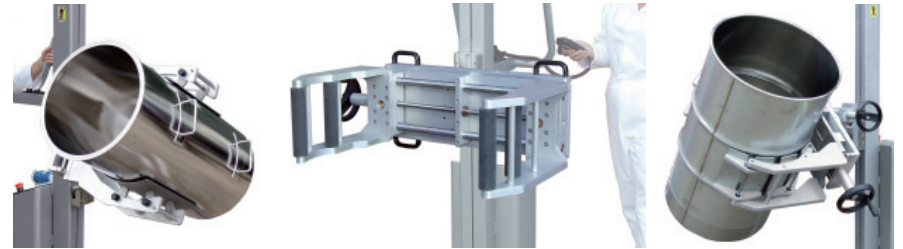
Drum and Reel Handling Vertical to Horizontal Via the External Diameter
